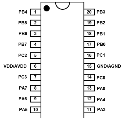
PMS123- H20:HTSOP20 (150mil)
