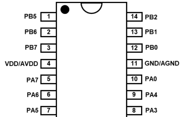
PMS123-S14: SOP14 (150mil)
