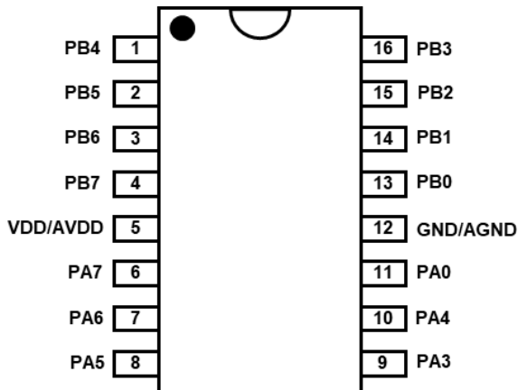
PMS123-S16: SOP16 (150mil)
