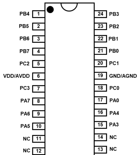
PMS123-Y24: SSOP24 (150mil)
